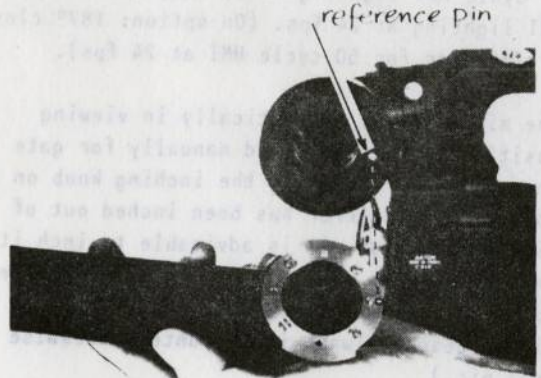
placing short and long eyepieces onto viewfinder
